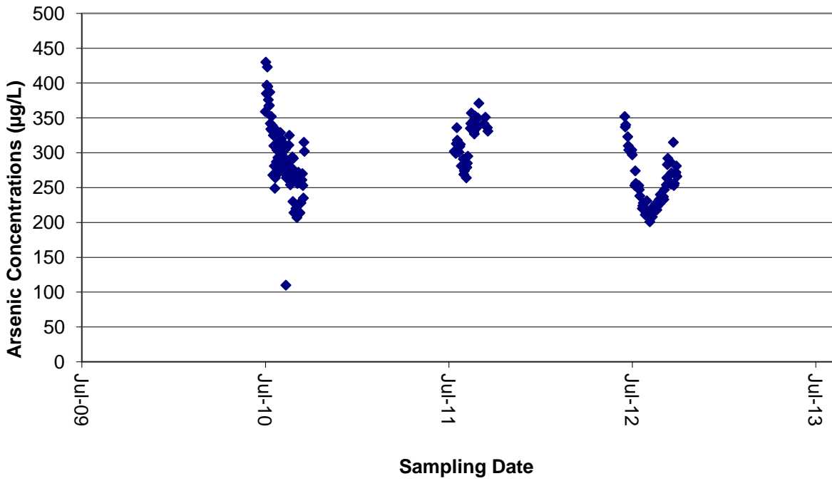
Dissolved Arsenic Concentrations at SNP 43-1 (2010 to 2012)
