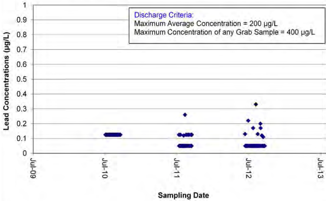
Total Lead Concentrations at SNP 43-1 (2010 to 2012)
