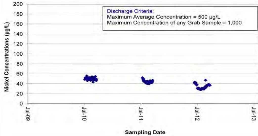
Total Nickel Concentrations at SNP 43-1 (2010 to 2012)
