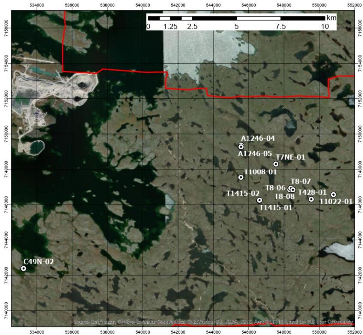
Figure 1: Plan map showing the location of the completed drillholes in August in relation to Diavik diamond mine.
