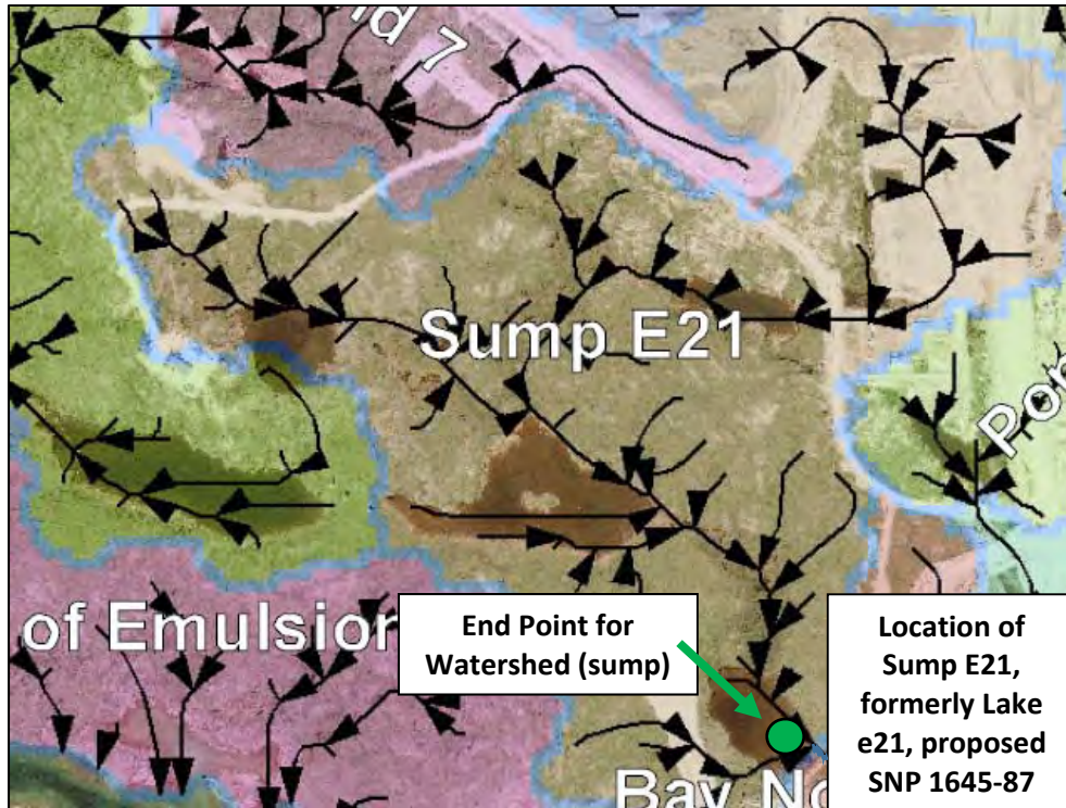
Figure 1 - Drainage basin for Sump E21 and proposed SNP station 1645-87. All drainage from WRSA-SCRP is expected to flow into Sump E21 and not travel beyond this point.
