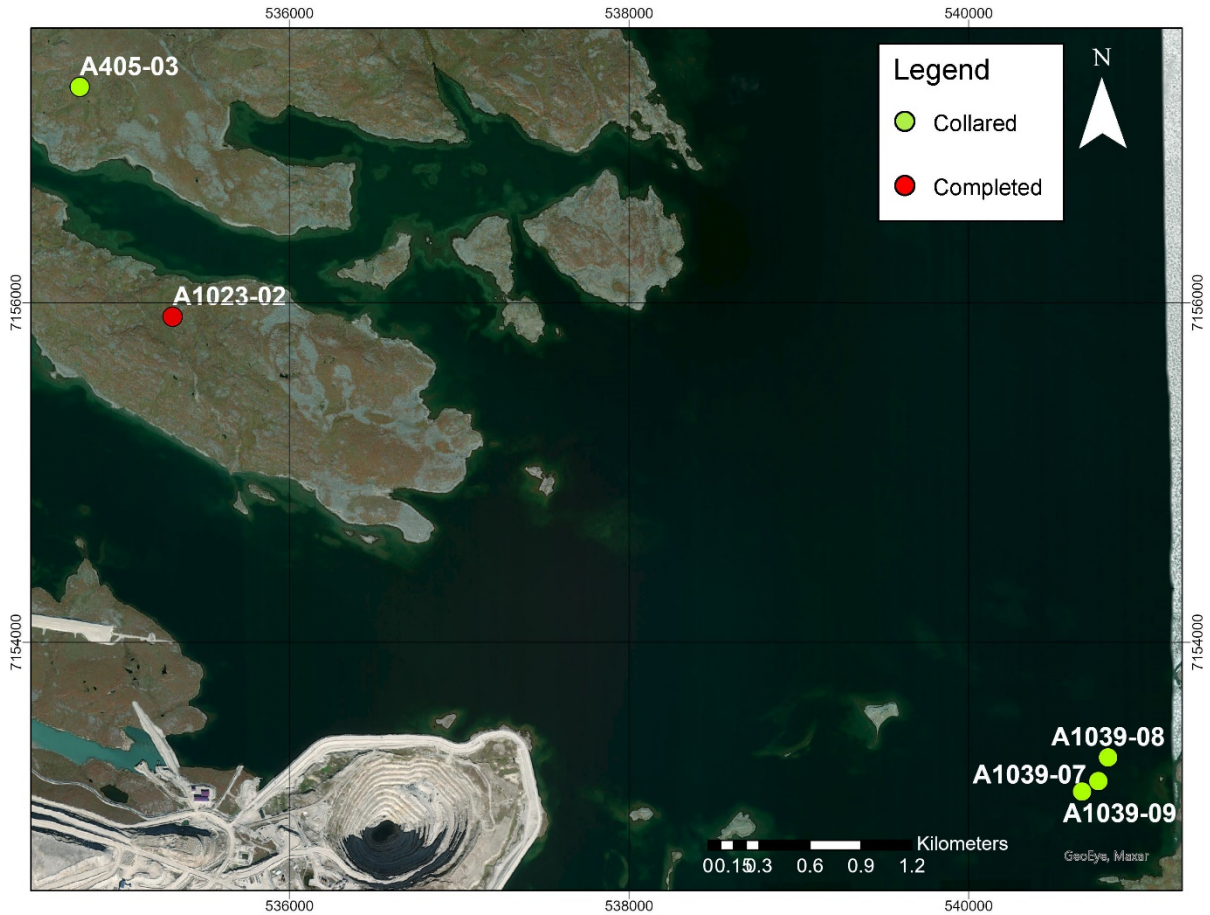
Figure 1: Plan map showing the one completed hole for the month of March (red dot). Also shown are 4 other holes that have been collared in anticipation of the drill.
